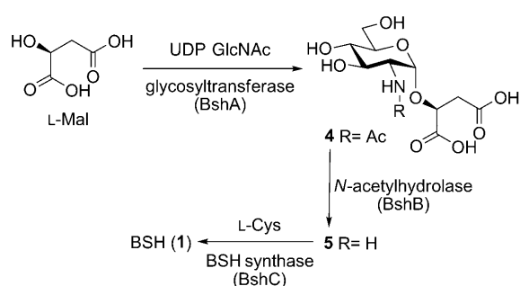
Figure 2. Biosynthetic pathway to bacillithiol (BSH, 1).
