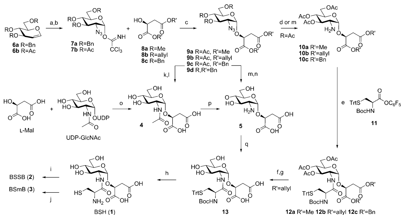
Scheme 1. Synthesis of BSH (1) along with its conversion into BSSB (2) and fluorescently labeled BSMB (3) is achieved by a route that also provides access to biosynthetic precursors 4 and 5. Reagents and conditions: a) CAN (2.6 equiv), NaN 3 (2.0 equiv), CH 3 CN, then H 2 O; b) NaH, Cl 3 CCN, THF, 0°C, 7a 24% and 7b 67% over two steps; c) Me 3 SiOTf (0.5 equiv), CH 2 Cl 2 , –30°→–10°C, 3–5 h, 9a 72% (only \alpha ), 9b 84% ( \alpha : \beta 95:5), 9c 90% ( \alpha : \beta 96:4), 9d 37% ( \alpha : \beta 31:69); d) Ph 3 P (3 equiv), THF, H 2 O (8:1), room temperature, 15 h; e) 11 (1.2 equiv), HOBT (2 equiv), Et 3 N (2 equiv), DMF, room temperature, 6–18 h, 12a 66%, 12b 35%, 12c 37% over two steps; f) [Pd(PPh 3 ) 4 ] (10 mol%), imidazole (10 equiv), THF, room temperature, 14 h; g) NaOMe, MeOH, 0°C, 75 min, 68% over two steps; h) TFA, Et 3 SiH, CH 2 Cl 2 (80:2:20), 0°C, 20 min, 99%; i) aq NH 4 HCO 3 , 1 h, 99%; j) mBBR, NaHCO 3 , CH 3 CN, H 2 O, 2 h, 90%; k) Ac 2 O, Pd/C, Et 3 SiH, EtOAc, room temperature, 12 h; l) NaOMe, MeOH, 0°C, 50% over two steps; m) Pd/C, H 2 (50 psi), EtOAc, aq HCl; n) NaOMe, MeOH, 0°C, 48% over two steps; o) BshA, L-malate, UDP-GlcNAc, 0.1 M NaCl, 10 mM MgCl 2 , 1 mM 2-mercaptoethanol, 25 mM HEPES pH 7.5, 20 h 37°C, 93%; p) BshB, pH 7, 23 h 37°C, 90%; q) 5, Boc-Cys(Trt)CO 2 H, HATU, Et 3 N, DMF, 15%. Abbreviations: DMF = N,N-dimethylformamide, HATU = 2-(1H-7-azabenzotriazol-1-yl)-1,1,3,3-tetramethyluronium hexafluorophosphate, HOBT = 1-hydroxybenzotriazole, UDP = uridine 5'-diphosphate, TFA = trifluoroacetic acid, Boc = tert -butoxycarbonyl, HEPES (buffer: 2-[4-(2-hydroxyethyl)-1-piperazinyl]ethanesulfonic acid), CAN = cerium(IV) ammonium nitrate, OTf = triflate (CF 3 SO 3 ).
